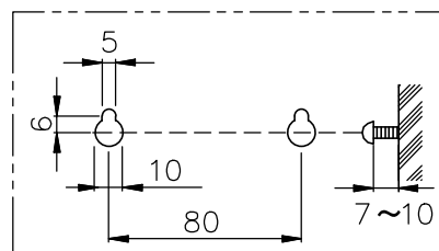
Hanging holes dimension diagram
